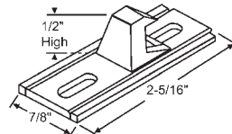
12-308 Black Plastic Peachtree
