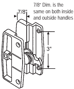
14-95 Handle Assembly Columbia
