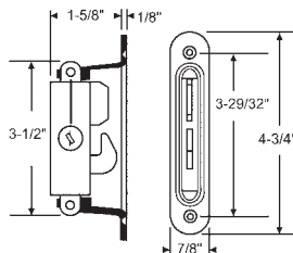
900-18867 Diagonal Hub. Aluminum Finish Use: 900-14560 for Keeper Traco
