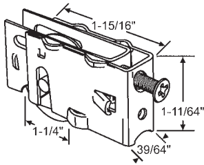
900-10095 Max. Dimple Width 13/16" Betterbilt
