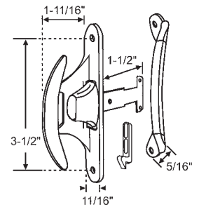
14-155A Includes Keeper Bayform
