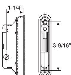
16-443 Mortise Lock and Plate
