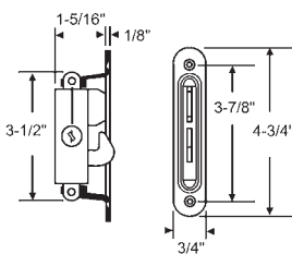
900-9169 Diagonal Hub. Aluminum Finish
