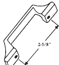
91-90 Mounting Holes Tapped 10-24
