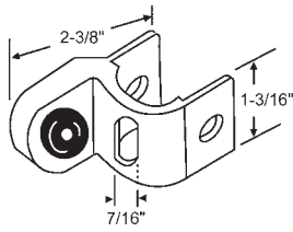
91-5 Inswing/Outswing for Concealed Latch with Round Bar
