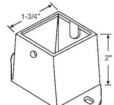
91-21 Pilaster Shoe for 1-3/4" Square Tube
