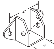
91-13 Headrail Bracket
