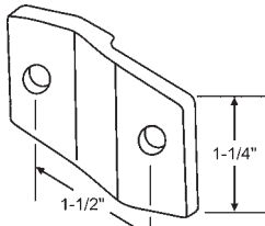
91-70 Alcove 1-1/4" Offset (1/8" per side). For all Size Posts
