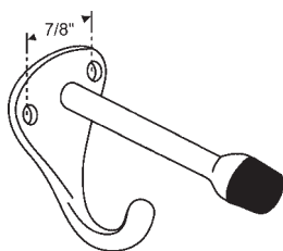
91-6 Coat Hook with Bumper 7/32" Hole Diameter
