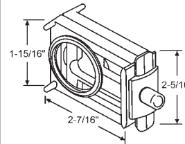
91-187 Zinc Die Cast - Unplated
