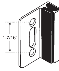
91-140 Inswing/Outswing for Concealed Latch
