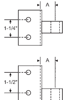
Part # A 91-2 1-5/64" Flushmetal
