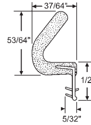
63-283BZ Door Weatherseal 97", Bronze
