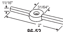
86-52 Propeller Style MALTA
