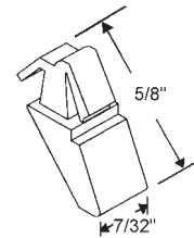
900-21058 Nylon Retainer NEWELL
